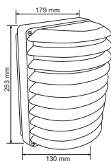
H-1190/S TALIN
