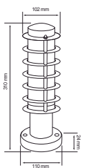
H-430/S AMSTERDAM
