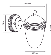
FTL-LED/006/N VEGA
