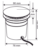
HLED-678/5W/30S CAIRO
