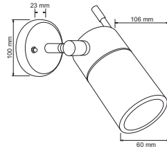
H-1105/S TROPEA
