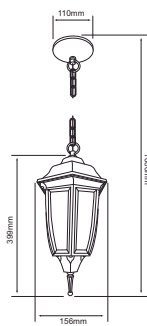
FTL-6003/N SANTIAGO
